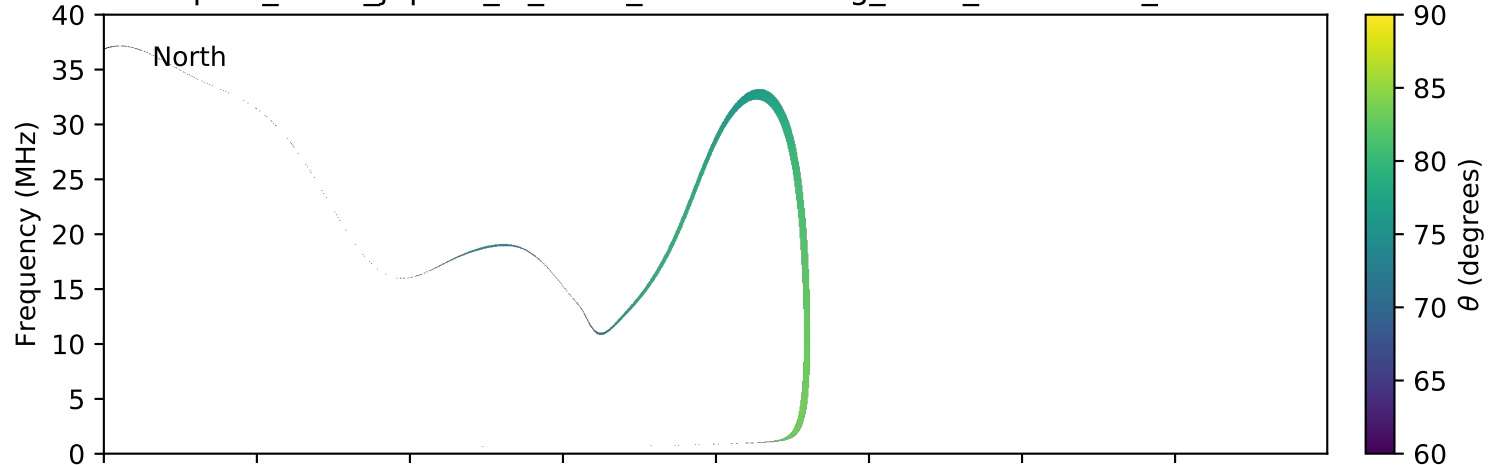
expres_earth_jupiter_io_isaac_lossc-wid1deg_3kev_20101224_v01.cdf
