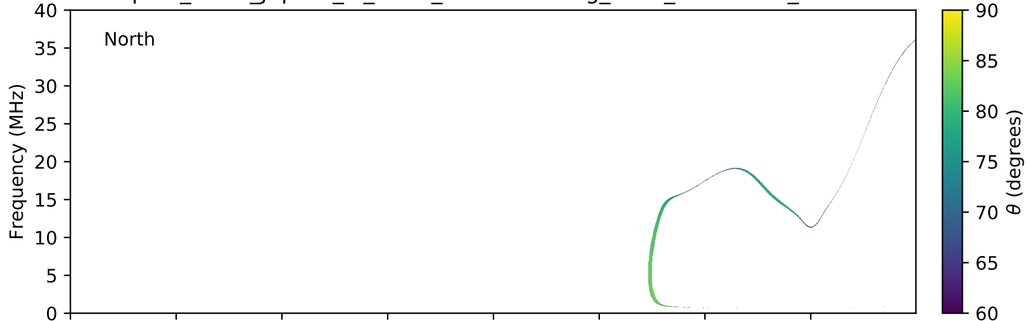
expres_earth_jupiter_io_isaac_lossc-wid1deg_3kev_20101223_v01.cdf
