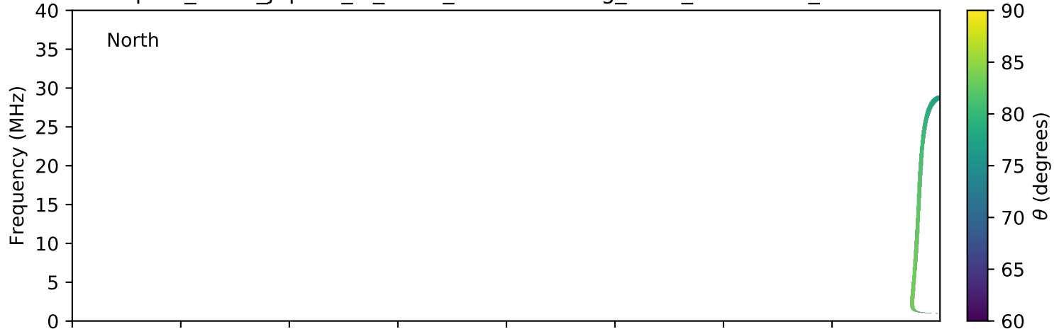
expres_earth_jupiter_io_isaac_lossc-wid1deg_3kev_20101221_v01.cdf
