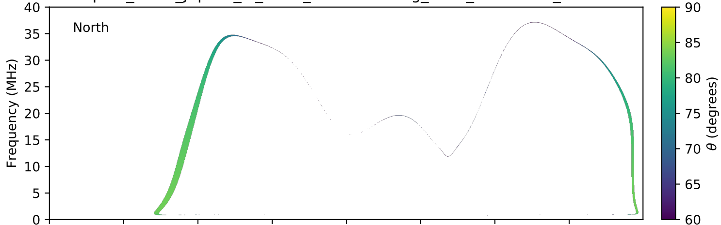
expres_earth_jupiter_io_isaac_lossc-wid1deg_3kev_20101220_v01.cdf
