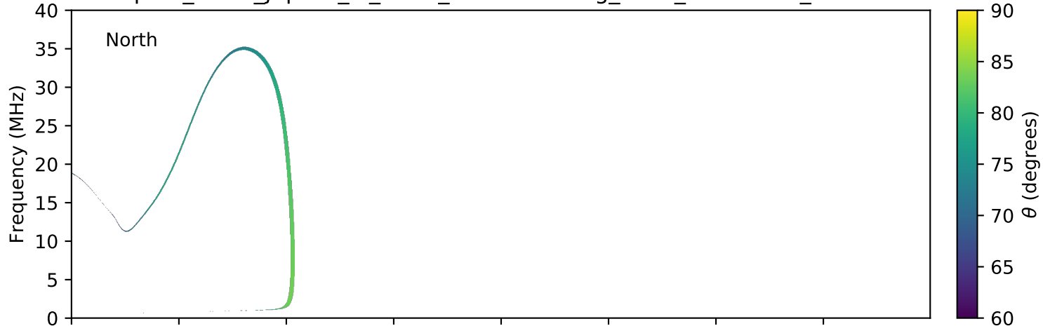
expres_earth_jupiter_io_isaac_lossc-wid1deg_3kev_20101219_v01.cdf
