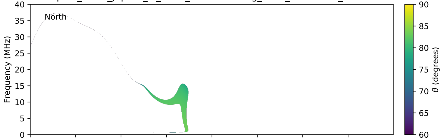
expres_earth_jupiter_io_isaac_lossc-wid1deg_3kev_20101217_v01.cdf
