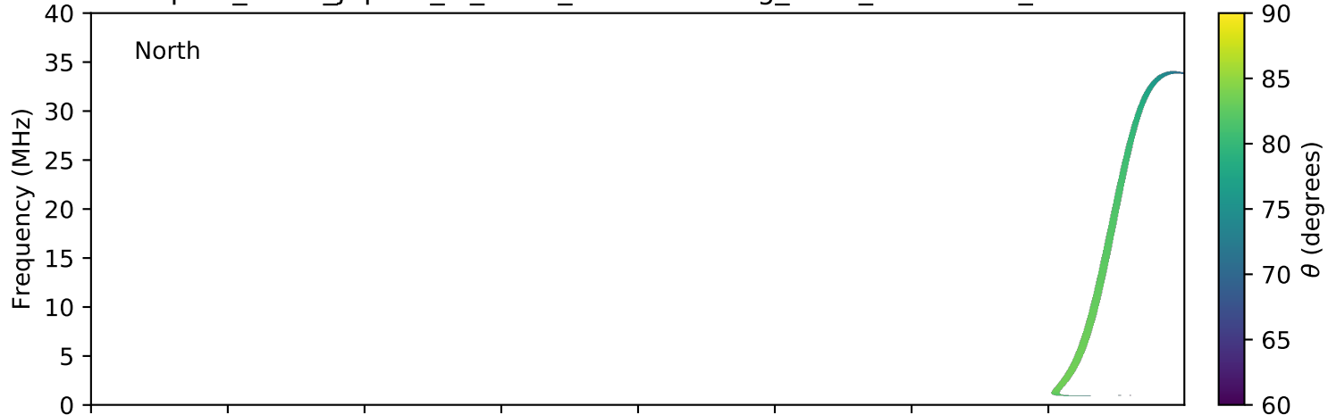
expres_earth_jupiter_io_isaac_lossc-wid1deg_3kev_20101214_v01.cdf
