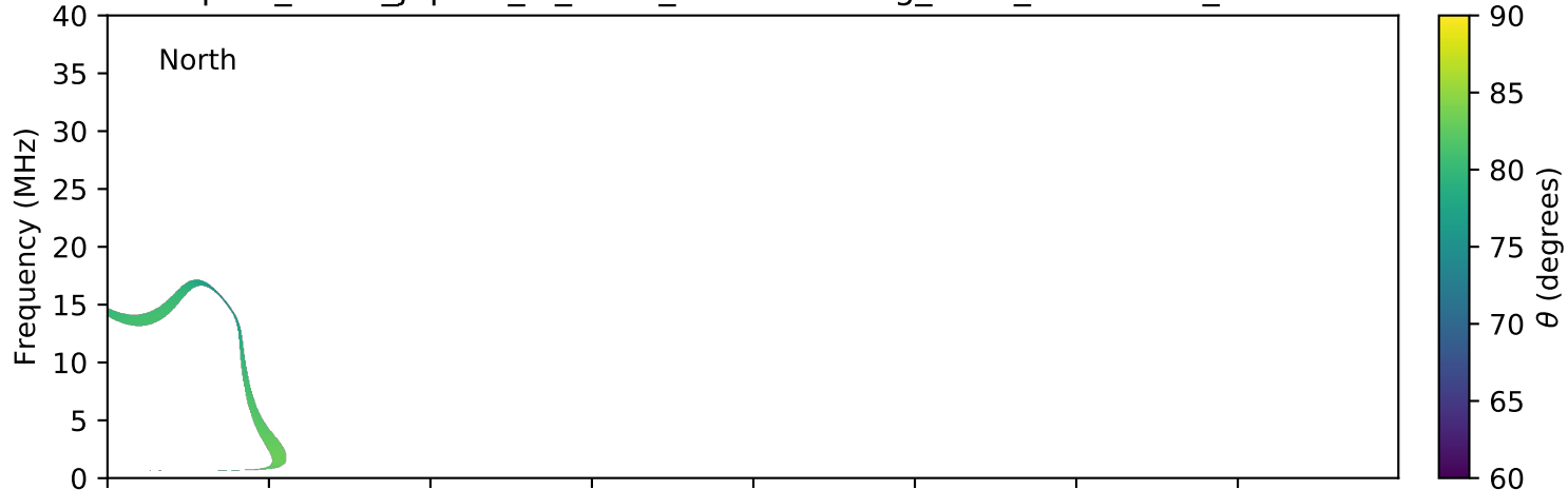
expres_earth_jupiter_io_isaac_lossc-wid1deg_3kev_20101212_v01.cdf
