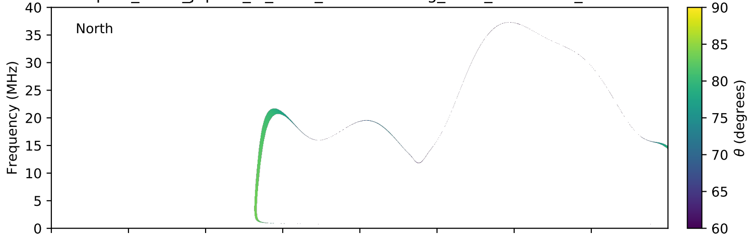
expres_earth_jupiter_io_isaac_lossc-wid1deg_3kev_20101211_v01.cdf
