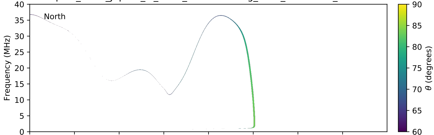
expres_earth_jupiter_io_isaac_lossc-wid1deg_3kev_20101208_v01.cdf
