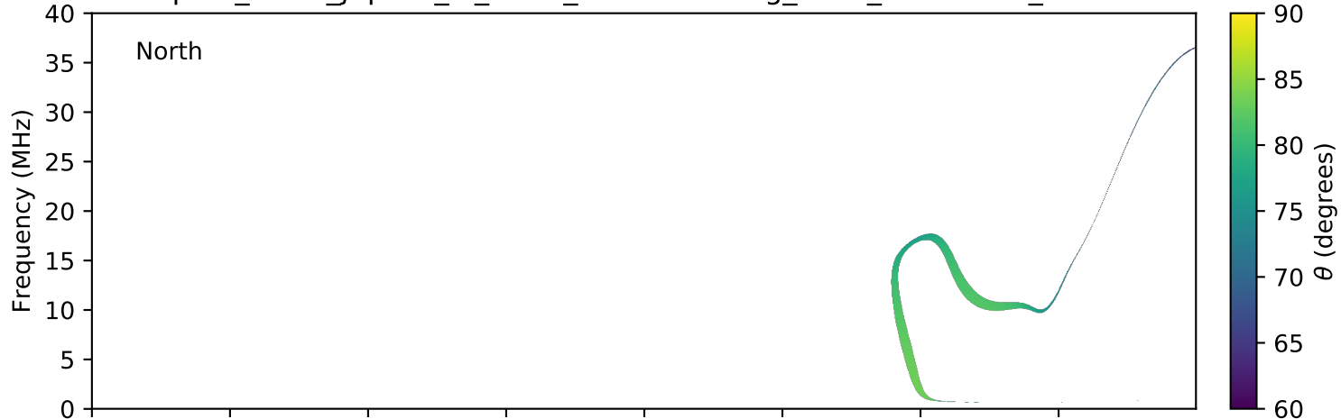
expres_earth_jupiter_io_isaac_lossc-wid1deg_3kev_20101207_v01.cdf
