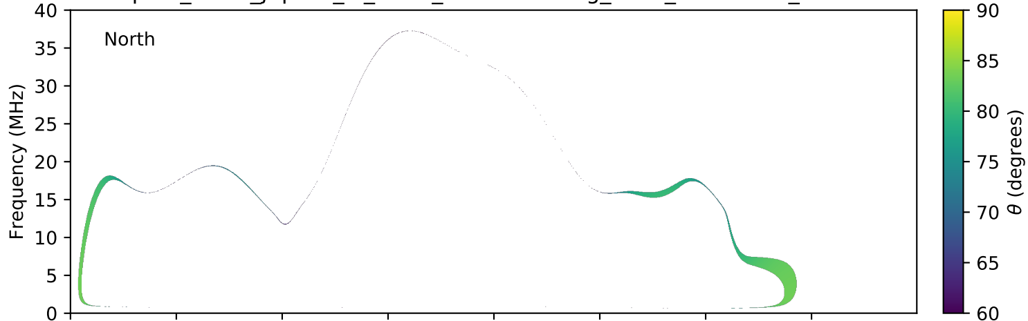
expres_earth_jupiter_io_isaac_lossc-wid1deg_3kev_20101206_v01.cdf
