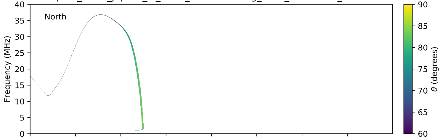
expres_earth_jupiter_io_isaac_lossc-wid1deg_3kev_20101203_v01.cdf
