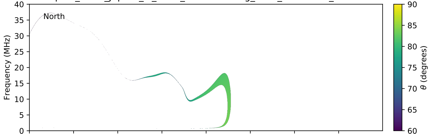
expres_earth_jupiter_io_isaac_lossc-wid1deg_3kev_20101201_v01.cdf
