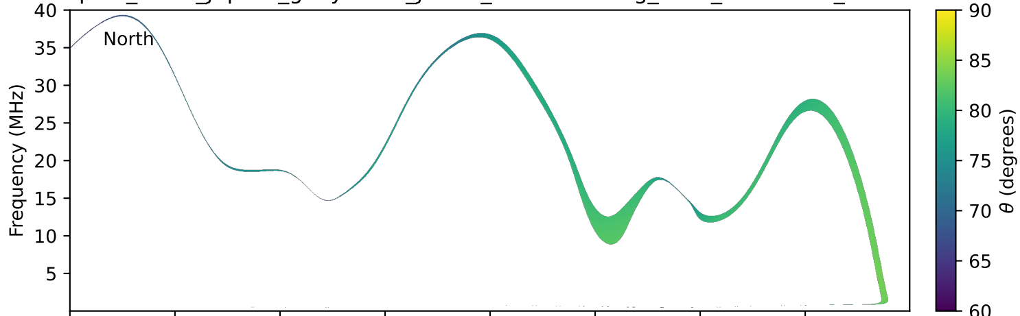
expres_earth_jupiter_ganymede_jrm33_lossc-wid1deg_3kev_20101228_v11.cdf
