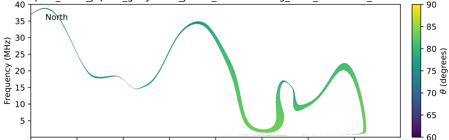
expres_earth_jupiter_ganymede_jrm33_lossc-wid1deg_3kev_20101221_v11.cdf
