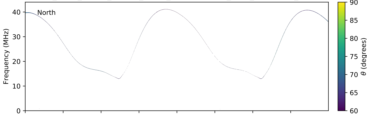
expres_earth_jupiter_europa_jrm09_lossc-wid1deg_3kev_20101230_v01.cdf
