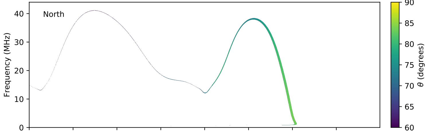
expres_earth_jupiter_europa_jrm09_lossc-wid1deg_3kev_20101227_v01.cdf
