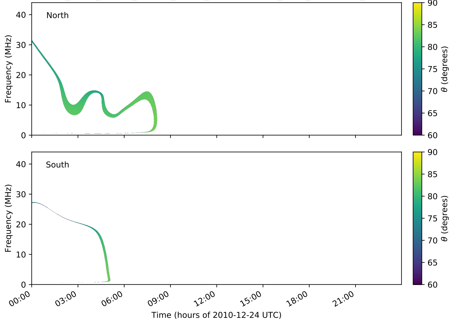
expres_earth_jupiter_europa_jrm09_lossc-wid1deg_3kev_20101224_v01.cdf
