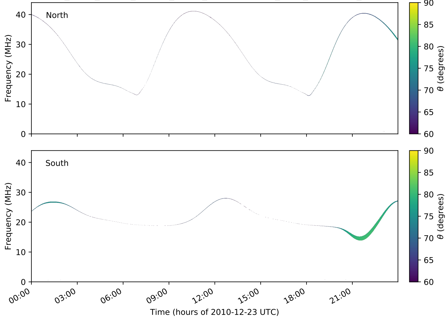
expres_earth_jupiter_europa_jrm09_lossc-wid1deg_3kev_20101223_v01.cdf
