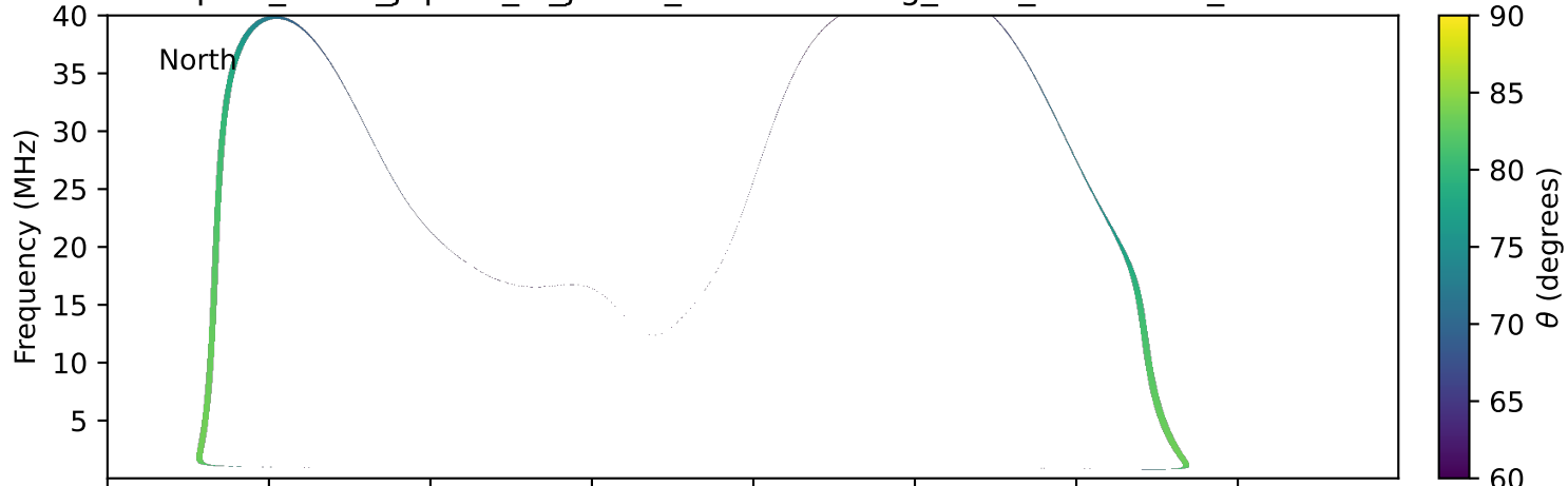
expres_earth_jupiter_io_jrm33_lossc-wid1deg_3kev_20101021_v11.cdf
