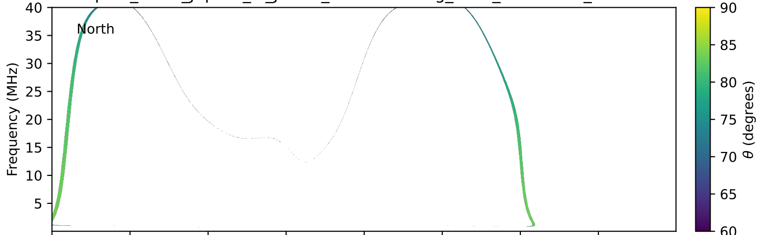
expres_earth_jupiter_io_jrm33_lossc-wid1deg_3kev_20101014_v11.cdf
