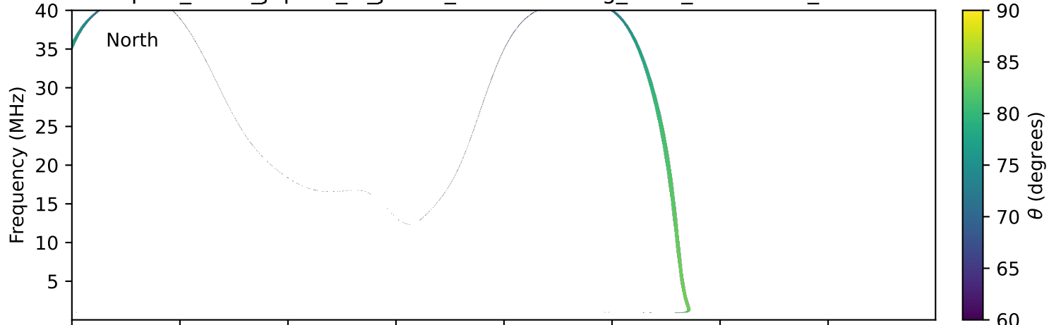
expres_earth_jupiter_io_jrm33_lossc-wid1deg_3kev_20101007_v11.cdf
