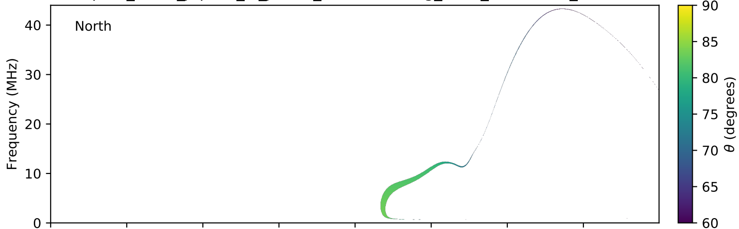
expres_earth_jupiter_io_jrm09_lossc-wid1deg_3kev_20101024_v01.cdf
