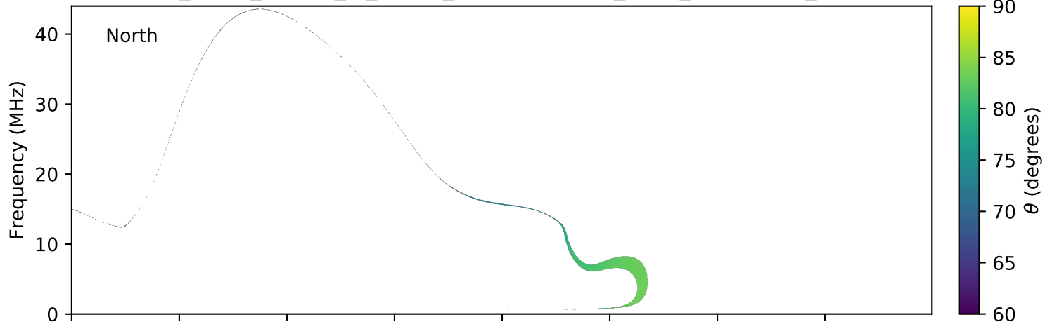
expres_earth_jupiter_io_jrm09_lossc-wid1deg_3kev_20101023_v01.cdf
