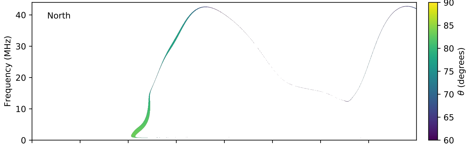
expres_earth_jupiter_io_jrm09_lossc-wid1deg_3kev_20101019_v01.cdf
