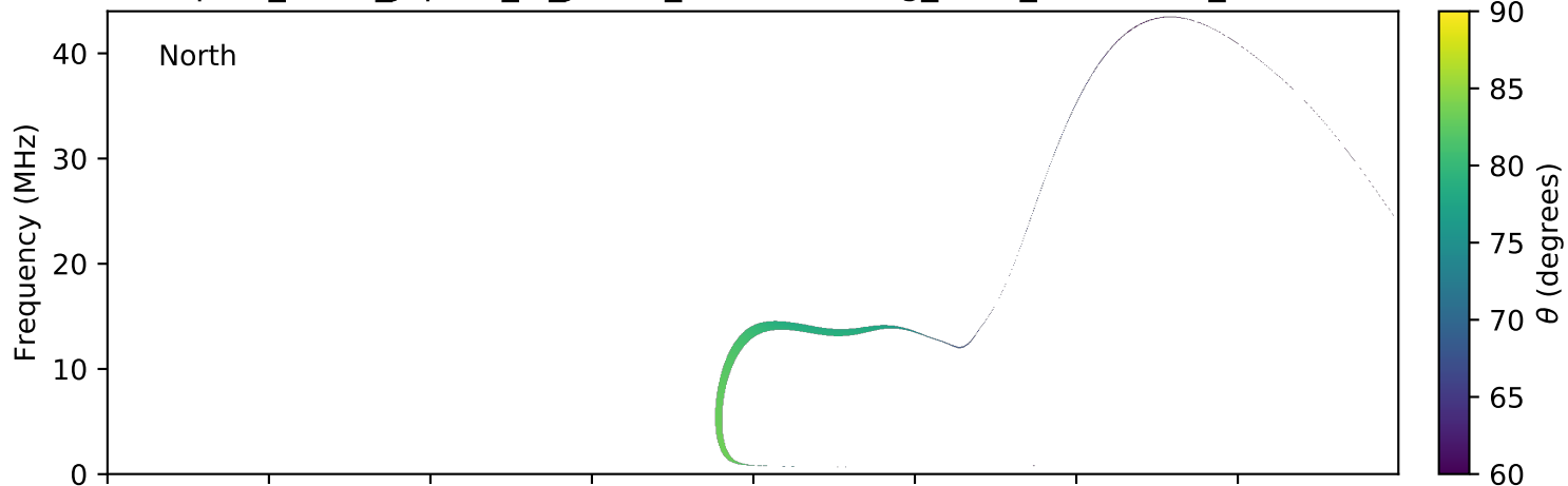
expres_earth_jupiter_io_jrm09_lossc-wid1deg_3kev_20101017_v01.cdf
