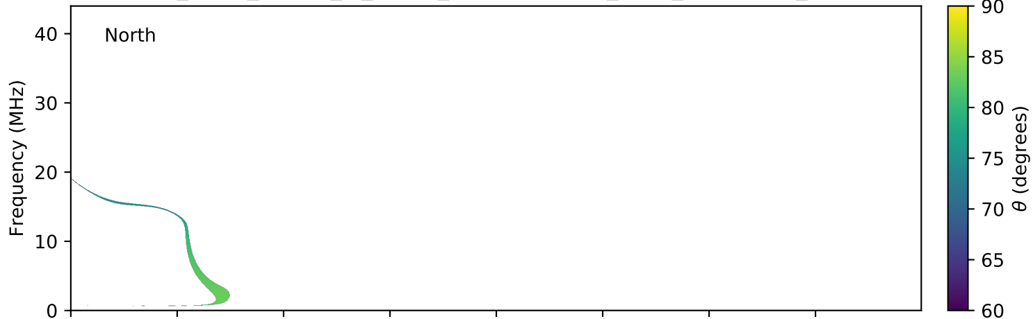
expres_earth_jupiter_io_jrm09_lossc-wid1deg_3kev_20101004_v01.cdf
