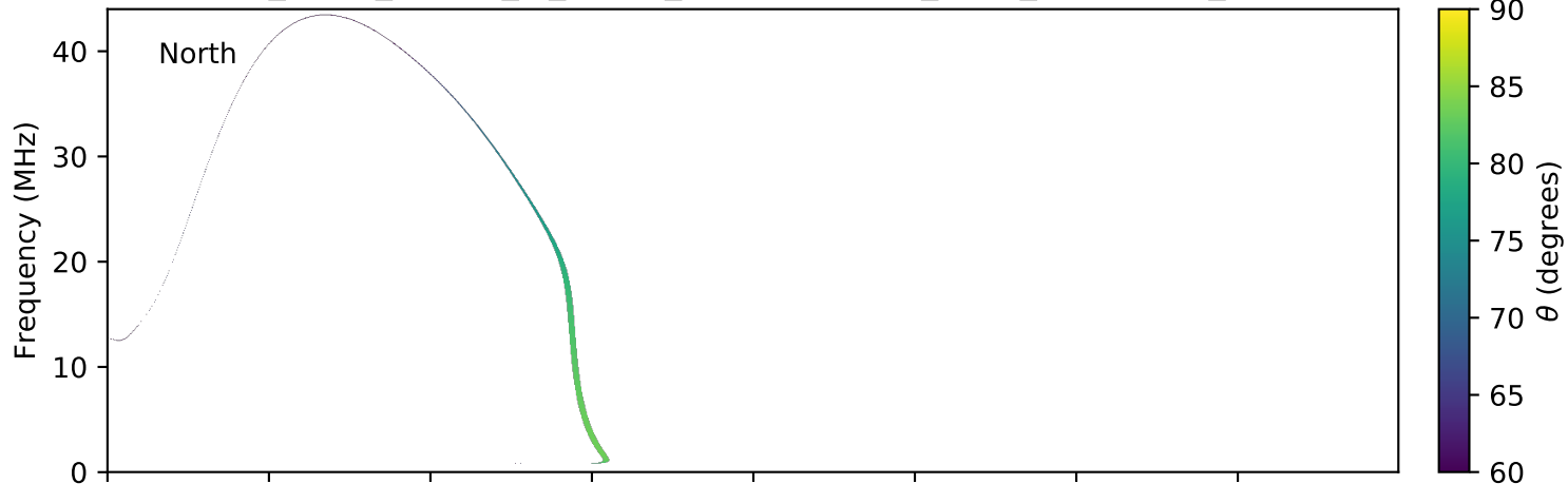
expres_earth_jupiter_io_jrm09_lossc-wid1deg_3kev_20101002_v01.cdf
