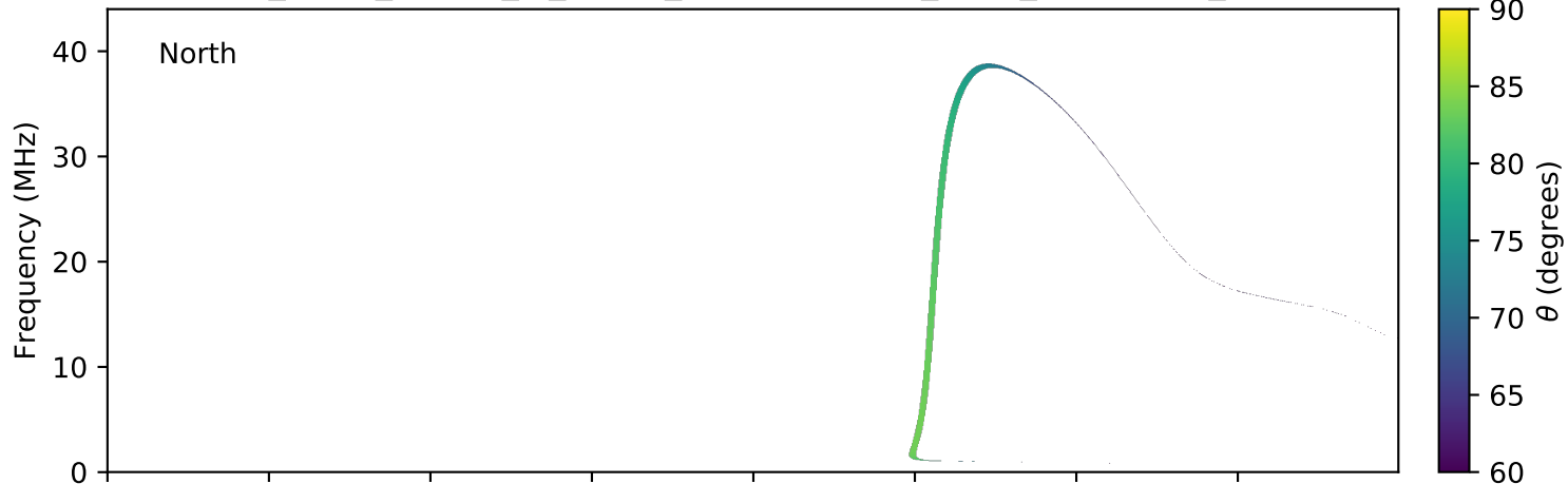
expres_earth_jupiter_io_jrm09_lossc-wid1deg_3kev_20101001_v01.cdf
