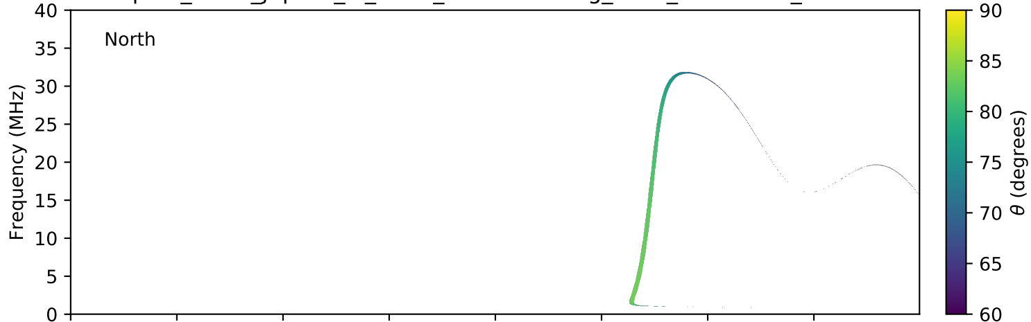
expres_earth_jupiter_io_isaac_lossc-wid1deg_3kev_20101031_v01.cdf
