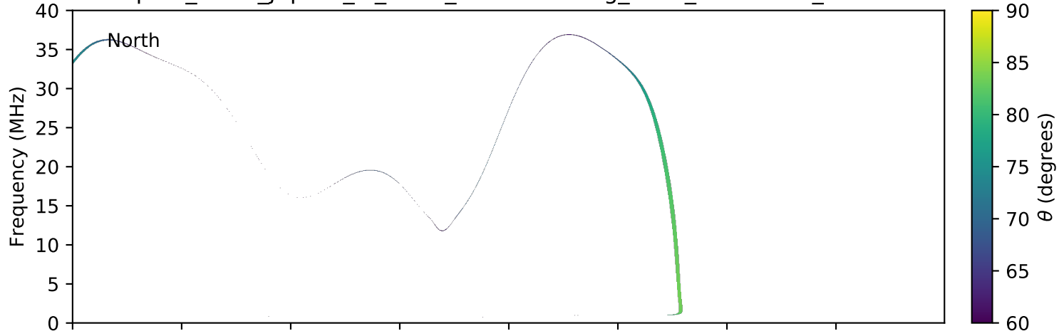
expres_earth_jupiter_io_isaac_lossc-wid1deg_3kev_20101030_v01.cdf
