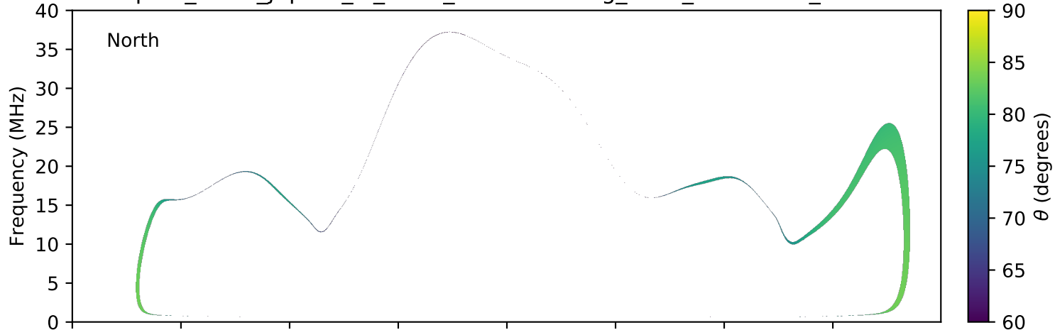
expres_earth_jupiter_io_isaac_lossc-wid1deg_3kev_20101028_v01.cdf
