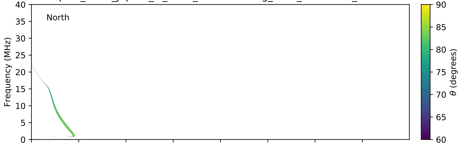
expres_earth_jupiter_io_isaac_lossc-wid1deg_3kev_20101027_v01.cdf
