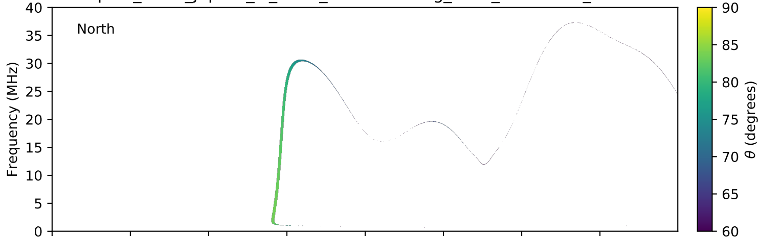
expres_earth_jupiter_io_isaac_lossc-wid1deg_3kev_20101026_v01.cdf
