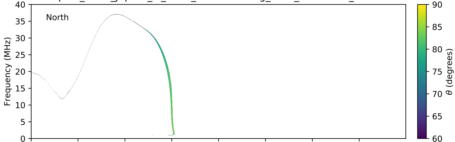
expres_earth_jupiter_io_isaac_lossc-wid1deg_3kev_20101025_v01.cdf
