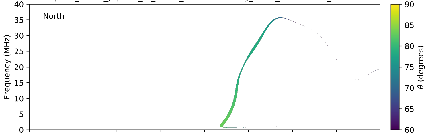
expres_earth_jupiter_io_isaac_lossc-wid1deg_3kev_20101024_v01.cdf
