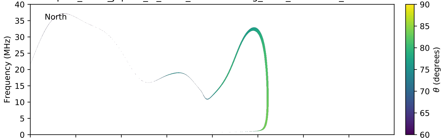
expres_earth_jupiter_io_isaac_lossc-wid1deg_3kev_20101023_v01.cdf
