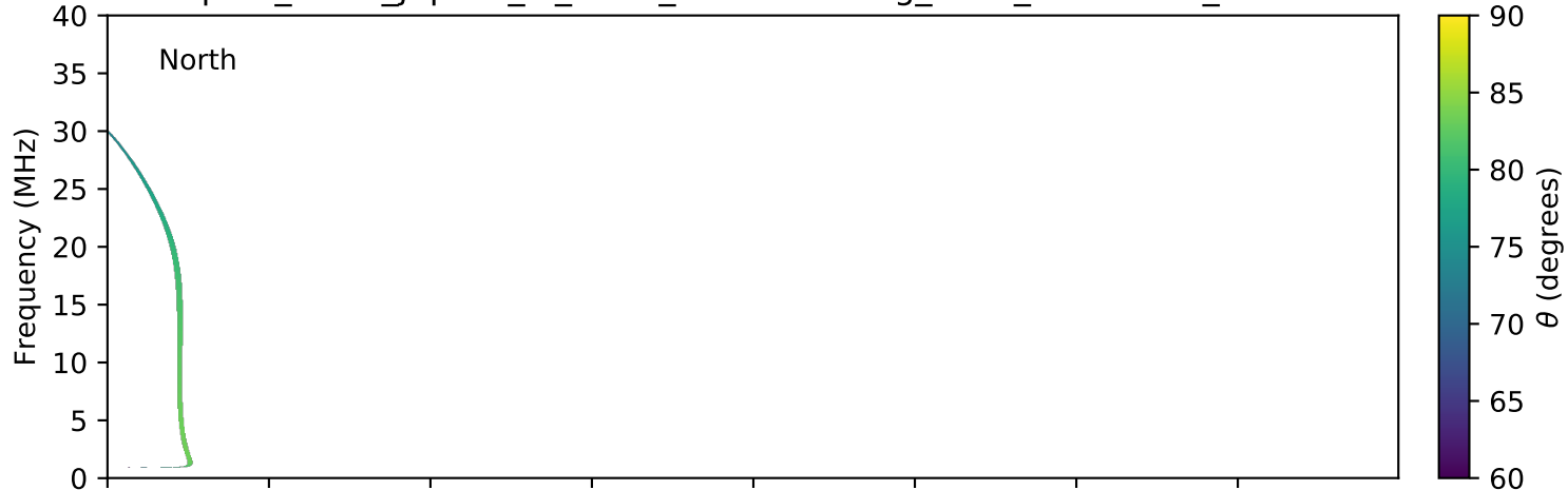
expres_earth_jupiter_io_isaac_lossc-wid1deg_3kev_20101020_v01.cdf
