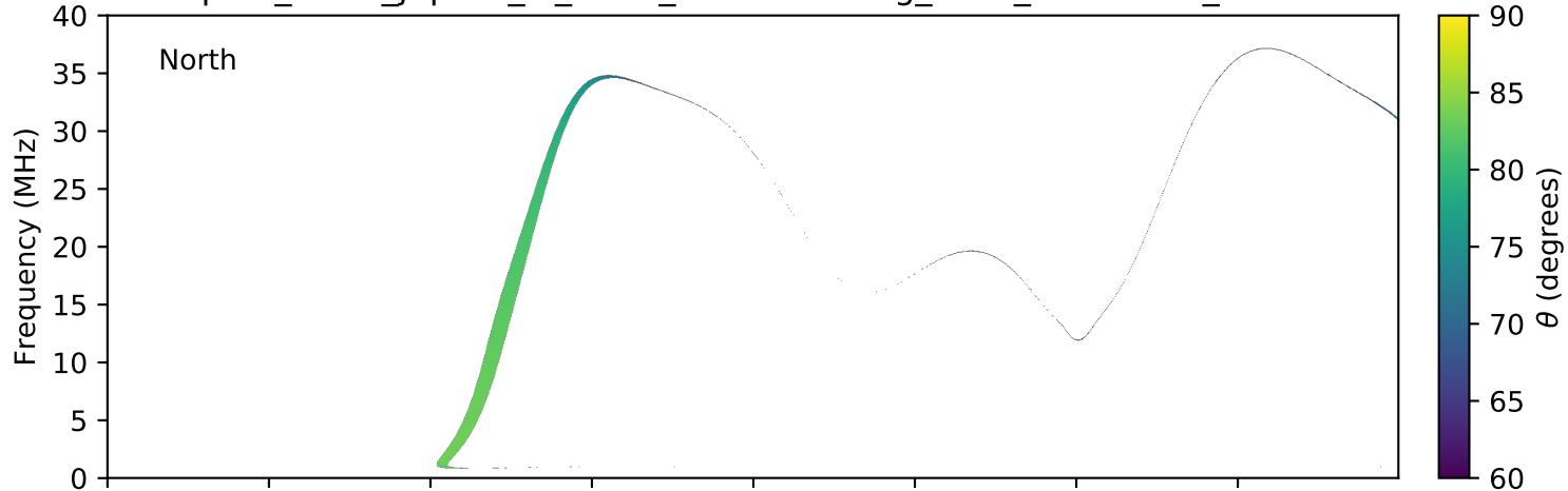
expres_earth_jupiter_io_isaac_lossc-wid1deg_3kev_20101019_v01.cdf
