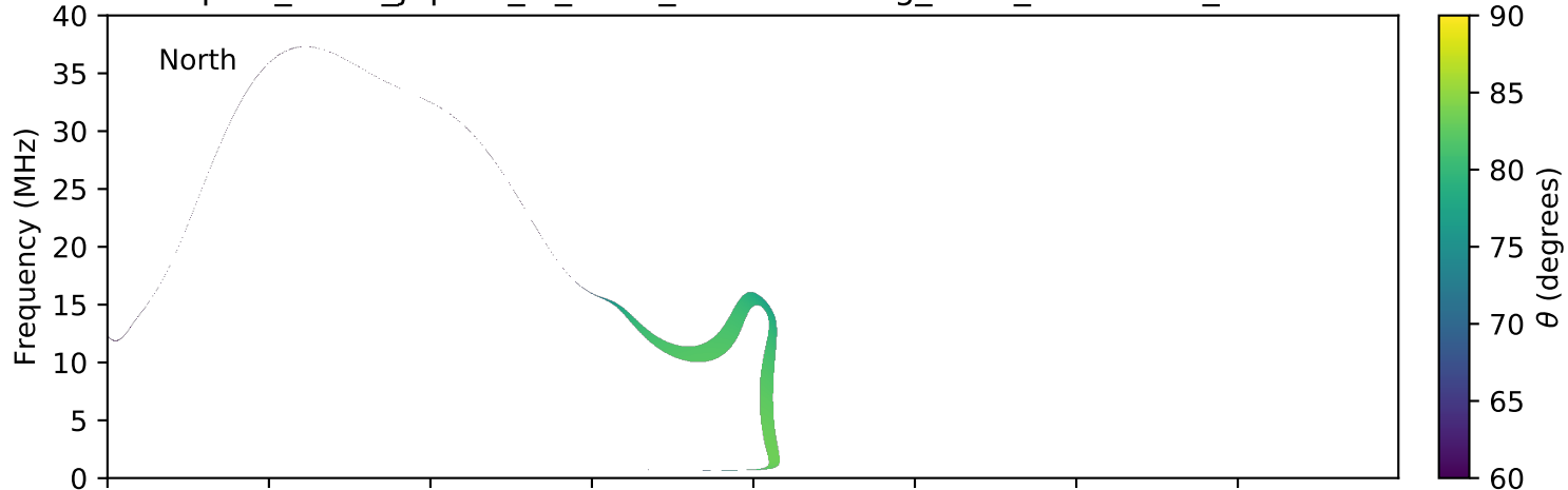
expres_earth_jupiter_io_isaac_lossc-wid1deg_3kev_20101016_v01.cdf
