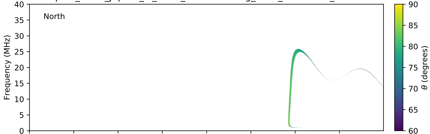
expres_earth_jupiter_io_isaac_lossc-wid1deg_3kev_20101015_v01.cdf
