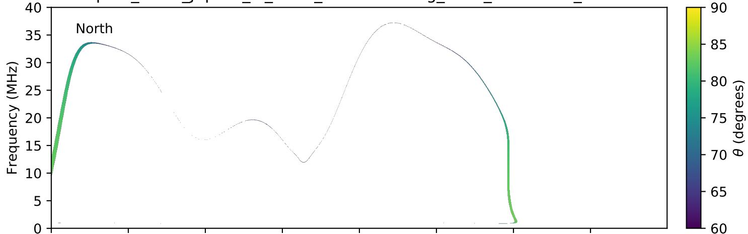
expres_earth_jupiter_io_isaac_lossc-wid1deg_3kev_20101014_v01.cdf
