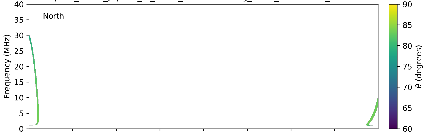
expres_earth_jupiter_io_isaac_lossc-wid1deg_3kev_20101013_v01.cdf
