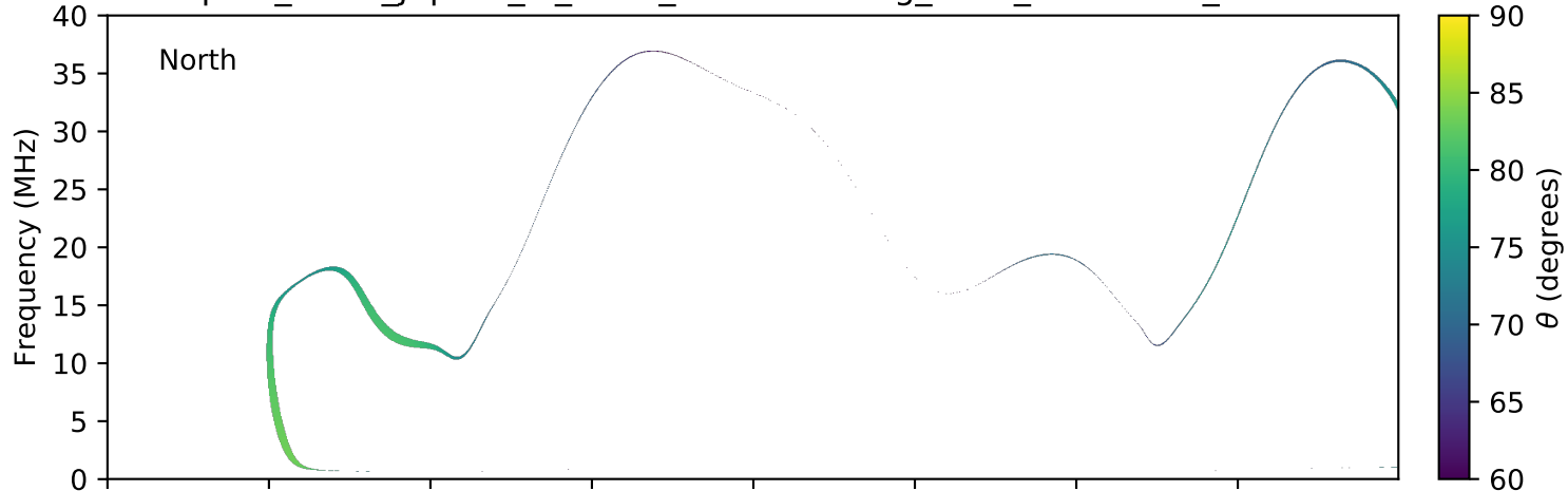
expres_earth_jupiter_io_isaac_lossc-wid1deg_3kev_20101012_v01.cdf
