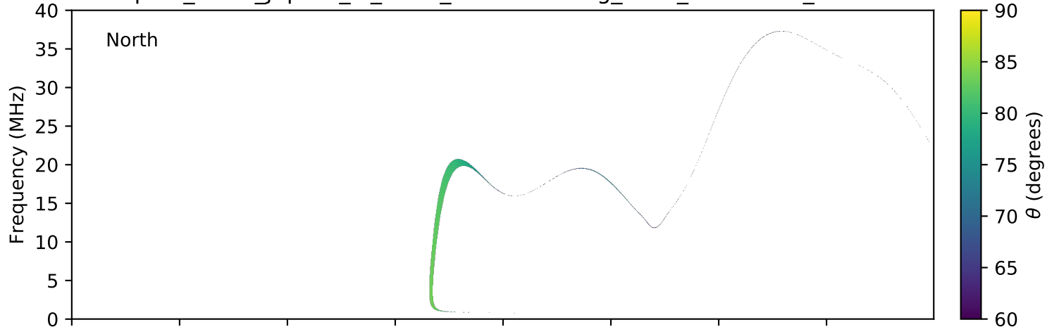
expres_earth_jupiter_io_isaac_lossc-wid1deg_3kev_20101010_v01.cdf
