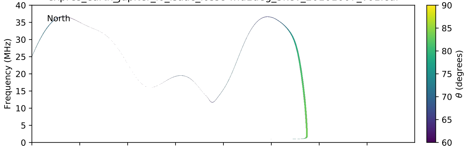
expres_earth_jupiter_io_isaac_lossc-wid1deg_3kev_20101007_v01.cdf
