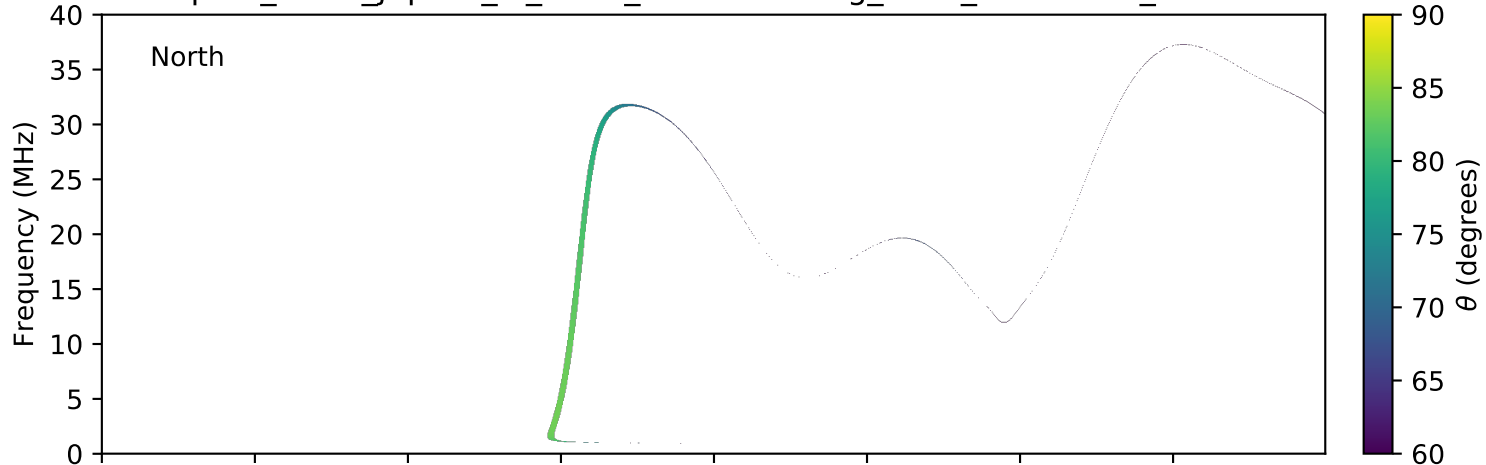
expres_earth_jupiter_io_isaac_lossc-wid1deg_3kev_20101003_v01.cdf
