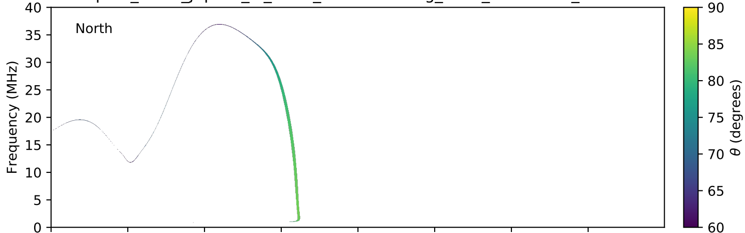
expres_earth_jupiter_io_isaac_lossc-wid1deg_3kev_20101002_v01.cdf
