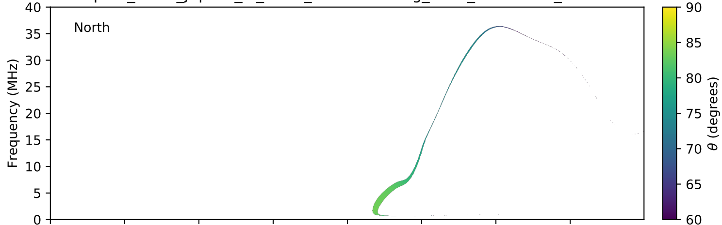
expres_earth_jupiter_io_isaac_lossc-wid1deg_3kev_20101001_v01.cdf
